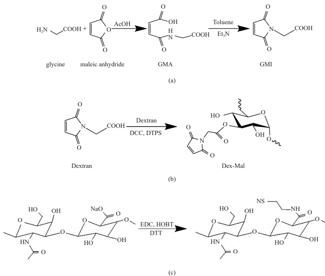
Figure 1. Reaction scheme for the syntheses of (a) GMI, (b) Dex-Mal and (c) HA-SH
