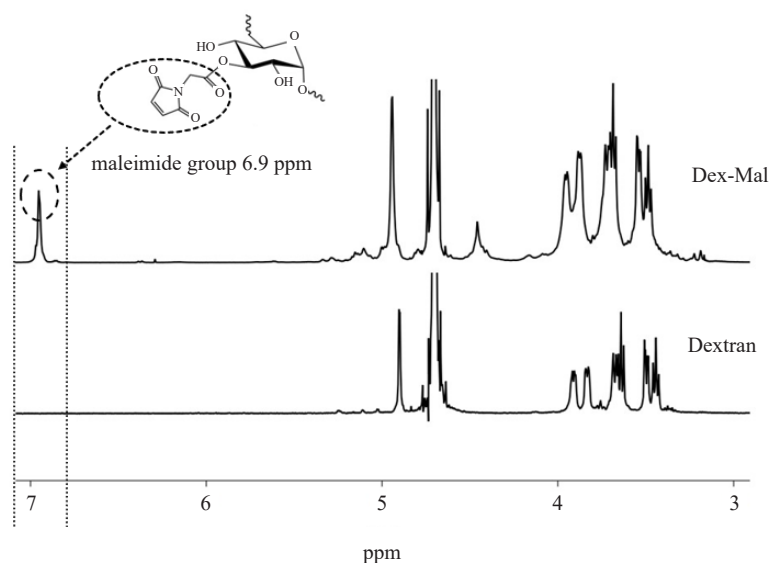
Figure 4. ^1\text{H} NMR spectrum of Dextran and Dex-Mal in \text{D}_2\text{O}
