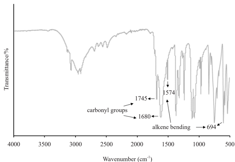
Figure 3. FTIR spectra of GMI
