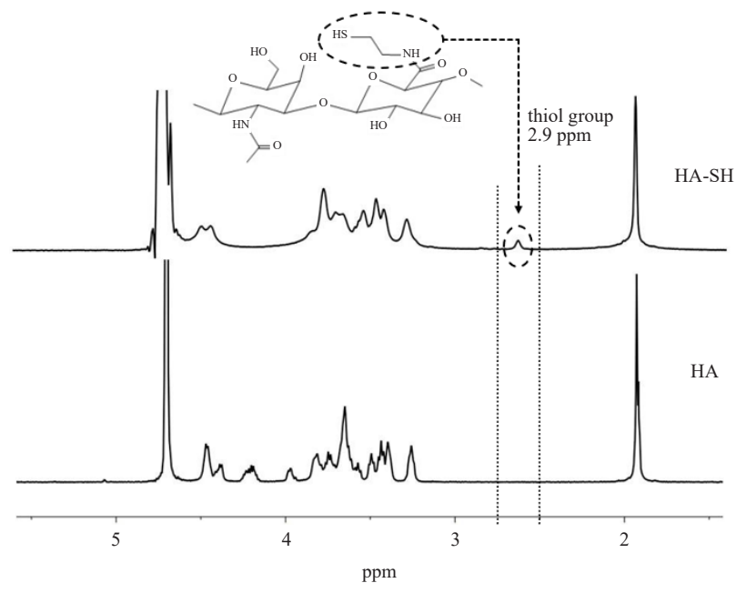
Figure 5. 1 H NMR spectra of HA-SH and HA in D 2 O
