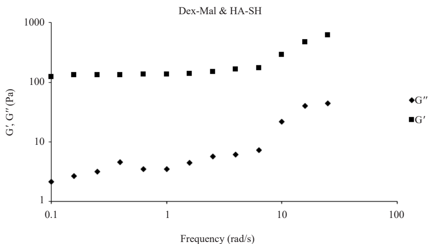
Figure 8. Frequency dependency of storage moduli ( G' ) and loss moduli ( G'' ) of the hydrogels
