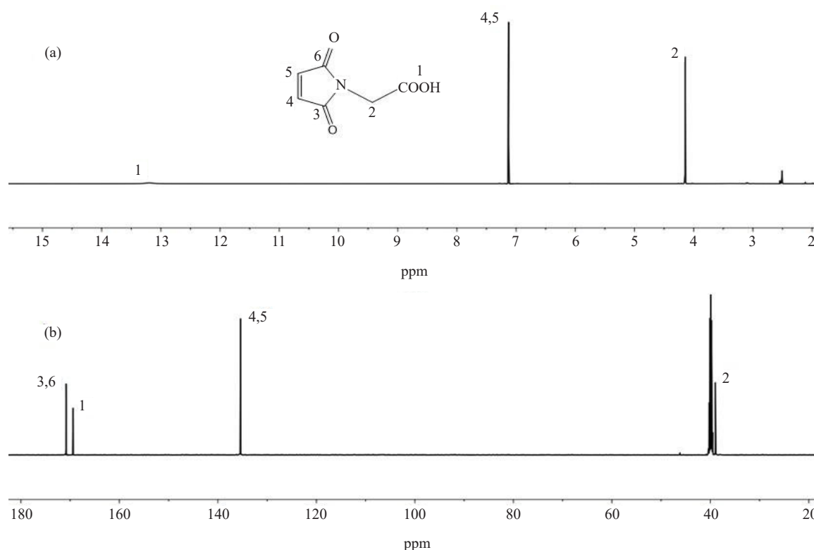
Figure 2. (a) ^1\text{H} and (b) ^{13}\text{C} NMR spectra of GMI in DMSO- d_6
